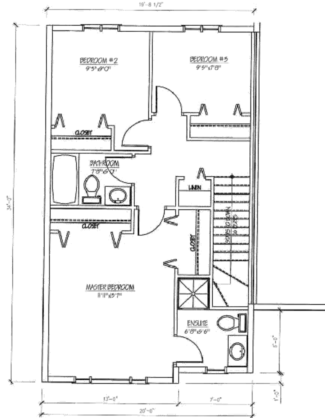
UPPER FLOOR PLAN SCALE: 3/16" = 1'-0"
