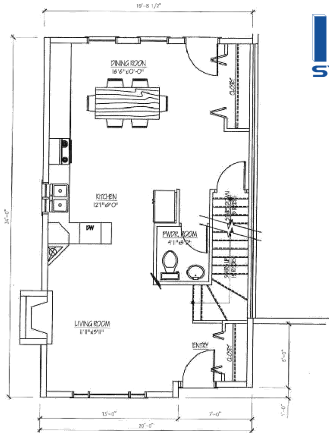
MAIN FLOOR PLAN SCALE: 3/16" = 1'-0"
